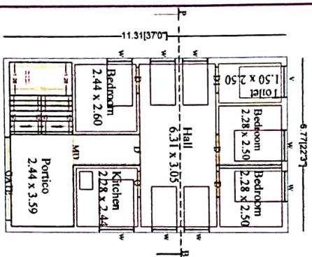
FLOOR-GROUND GROUND FLOOR PLAN
