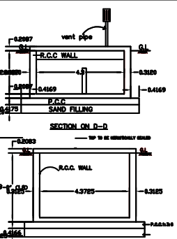
SECTION ON AA
