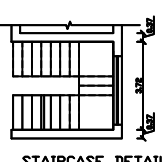
STAIRCASE DETAIL
