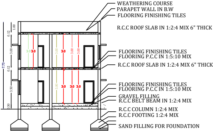
SECTION A TO B
