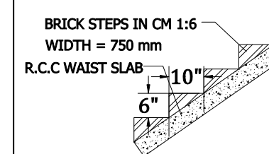
STAIRCASE DETAILS (NOT TO SCALE)
