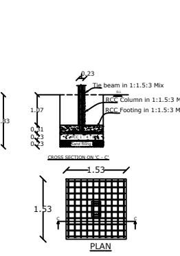
COLUMN FOUNDATION DETAILS:-
