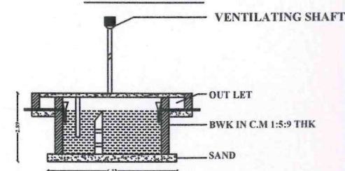
SEPTIC TANK
