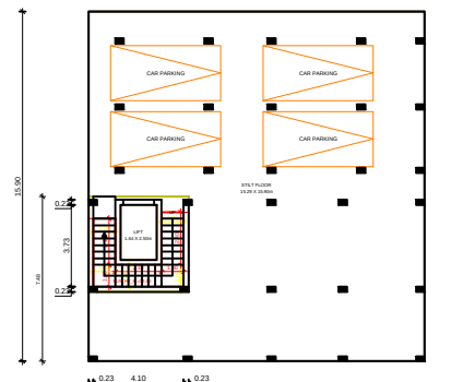
STILT FLOOR PLAN
