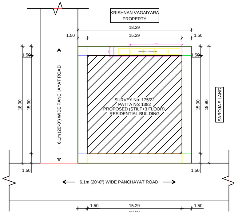
SITE PLAN
