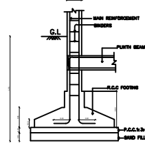
TYPICAL SECTION OF R.C.C. COLUMN FOUNDATION
