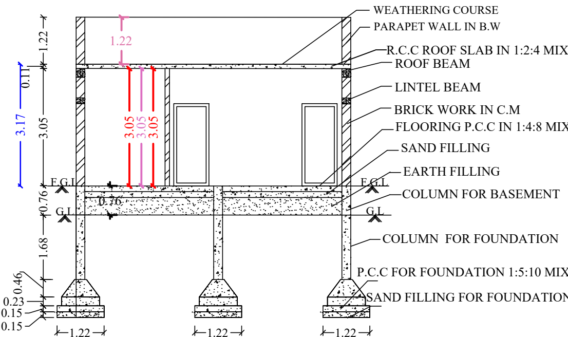
SECTION ON-AA
