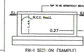
RW-1 SECTION (SAMPLE) RW_CAPACITY_L = 2000LTRS
