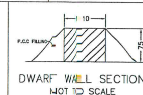
COMPOUND WALL DETAIL
