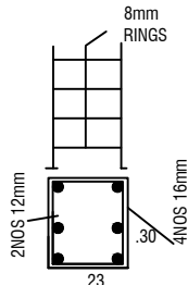
COLUMN DETAILS
