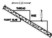
STAIRCASE DETAILS
