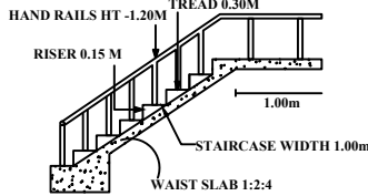
STAIRCASE DETAILS
