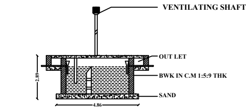
SEPTIC TANK
