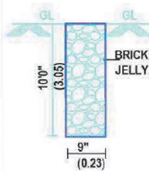
PERCOLATION PIT
