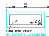
PLAN OF RWH_TANK
