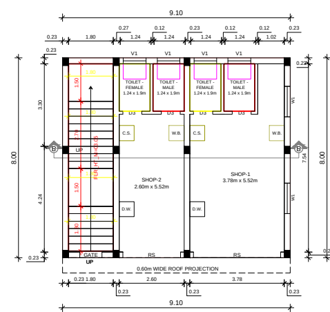
ALREADY APPROVED GROUND FLOOR PLAN
