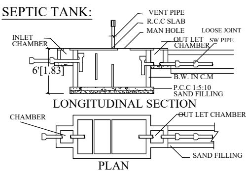
SEPTIC TANK:
