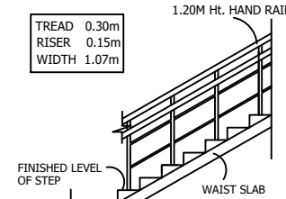
STAIRCASE DETAILS
