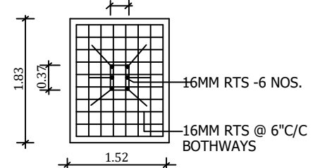
RAIN WATER RECHARGE PIT
