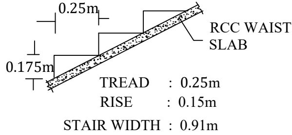
PRO. STAIRCASE DETAIL (NOT TO SCALE)
