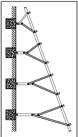
SOLAR PANEL:
