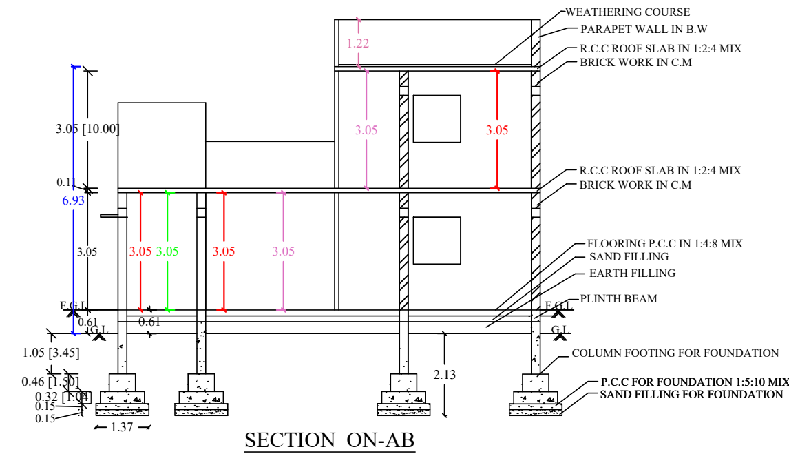
SECTION ON-AB
