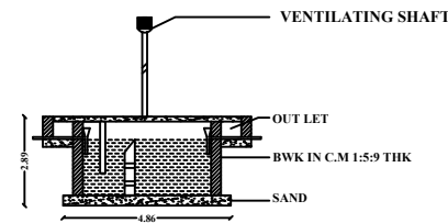
SEPTIC TANK
