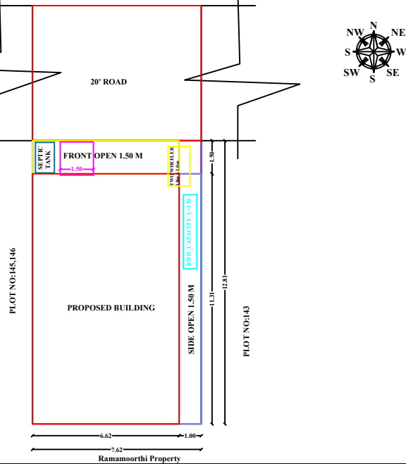
SEPTIC TANK
