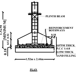
TYP.DET. COLUMN FOOTING
