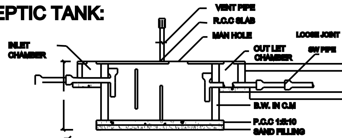
SEPTIC TANK:
