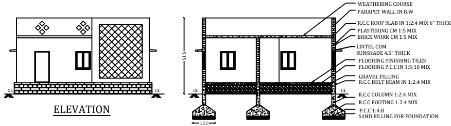
SECTION AB
