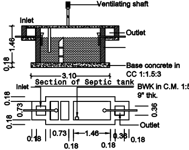
SEPTIC TANK DETAIL
