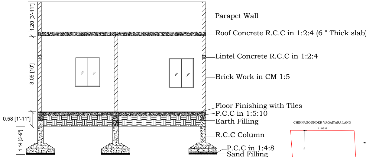
SECTION X-X
