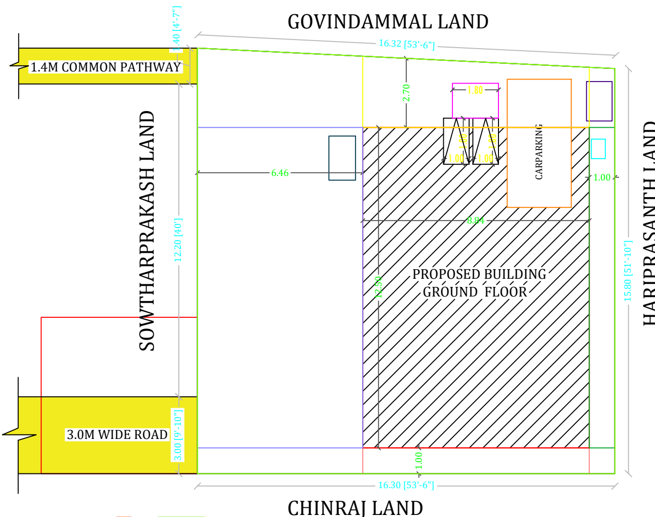
SITE PLAN
