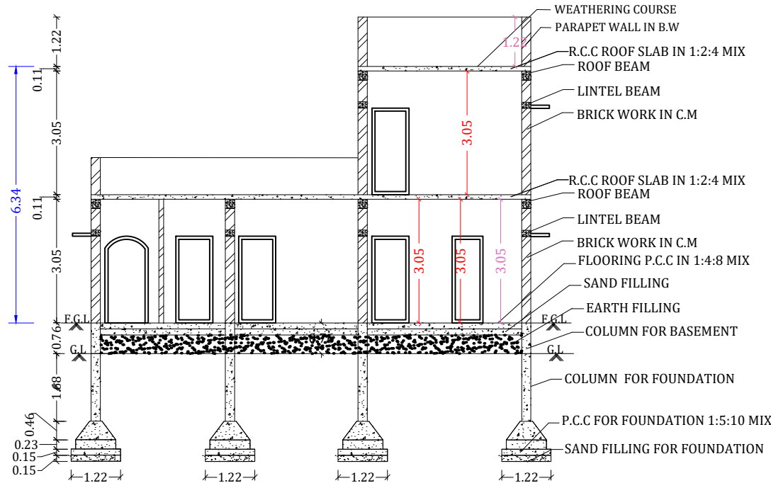
SECTION ON-AA
