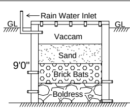
RAIN WATER HARVESTING TANK
