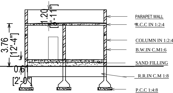
SECTION ON -XY
