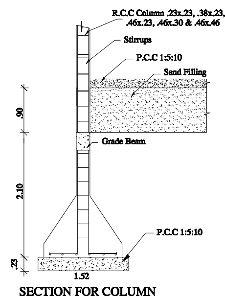
SECTION FOR COLUMN
