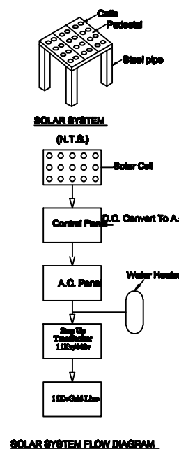
SOLAR SYSTEM FLOW DIAGRAM.
