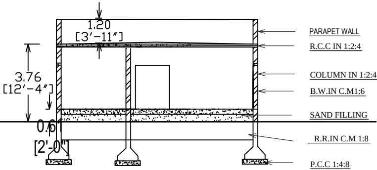
SECTION ON -XY
