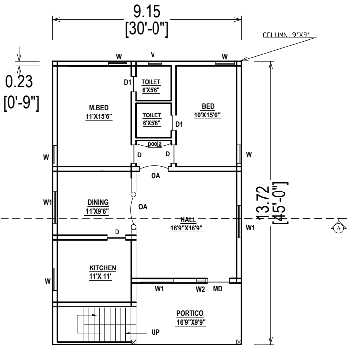
PLAN FACED TO EAST SCALE = 1:100
