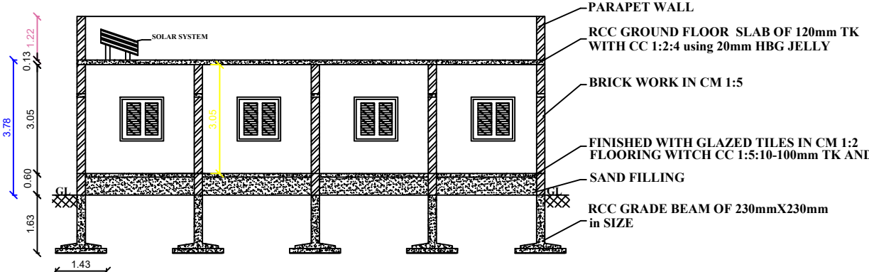
SECTION ON "BB"
