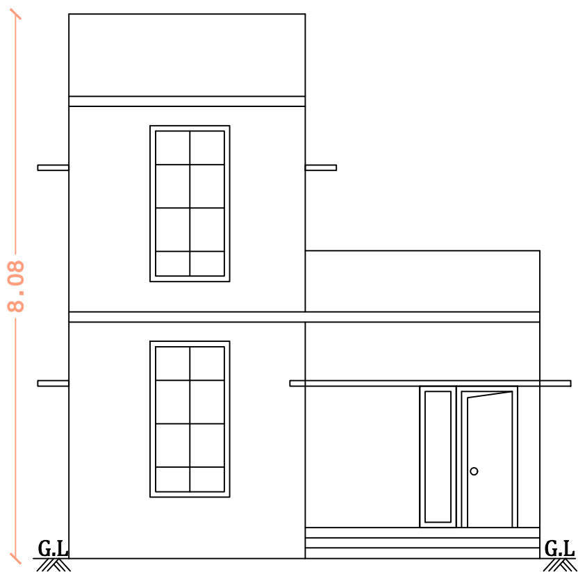
FRONT ELEVATION
