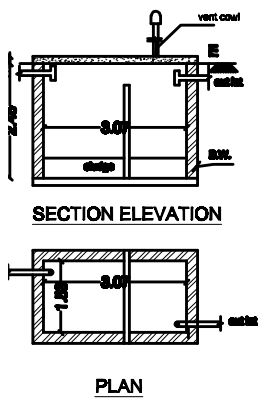
SEPTIC TANK
