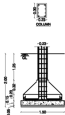
RCC COLUMN AND FOOTING
