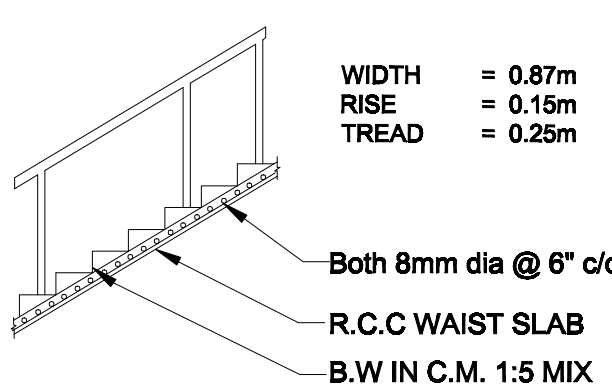
STAIRCASE DETAIL
