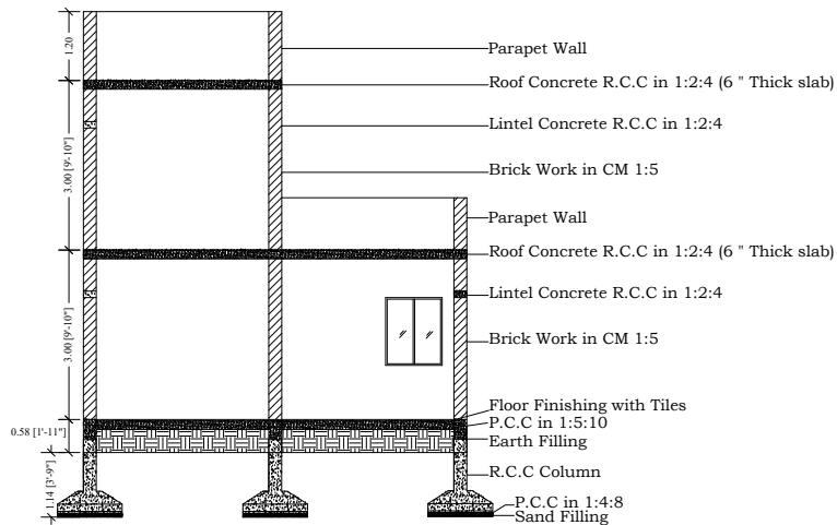
SECTION X-X
