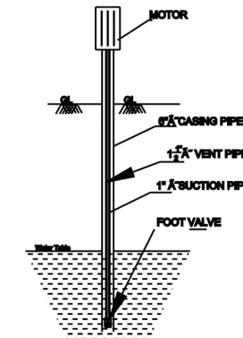
SEC. OF BOREWELL
