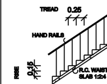
STAIRCASE DETAILS
