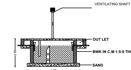
SEPTIC TANK
