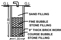
SECTION ON RAIN WATER COLLECTION TANK
