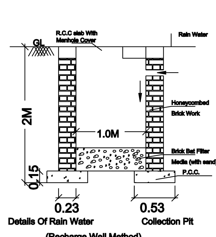
Details Of Rain Water (Recharge Well Method) SCALE:- 1"=4'0"
