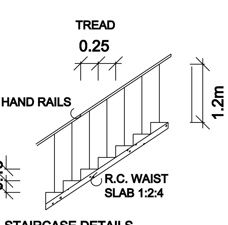
STAIRCASE DETAILS
