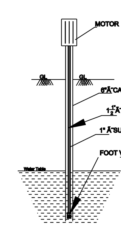
SEC. OF BOREWELL
