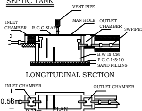
SECTION OF SEP.TANK
