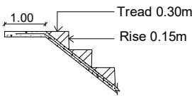
STAIRCASE DETAILS
