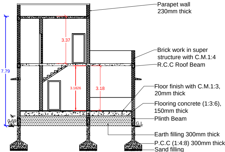
SECTION AT "AA"
