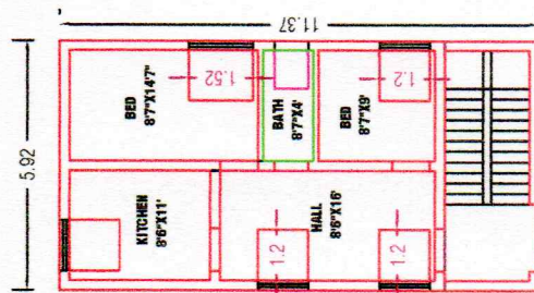
FLOOR-FIRST PROPOSED FIRST FLOOR PLAN
