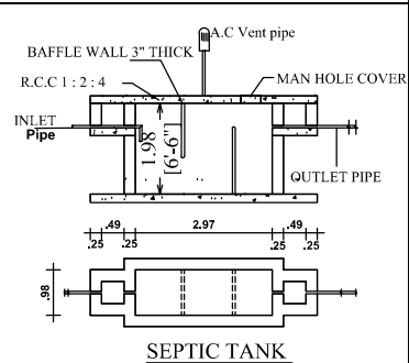
SEPTIC TANK
