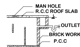
SECTION ON-AA
