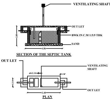
SEPTIC TANK
