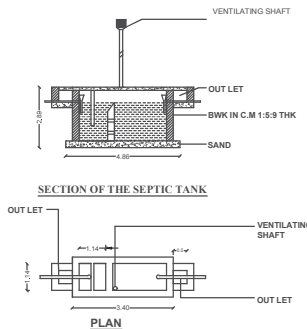
SEPTIC TANK
