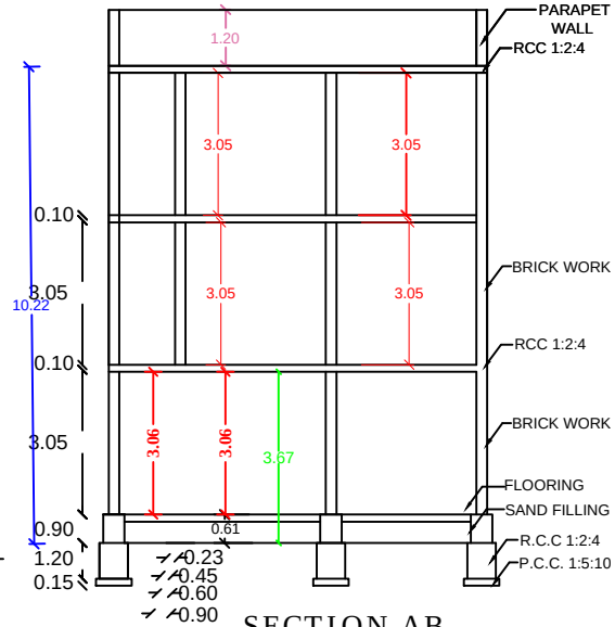
SECTION AB
