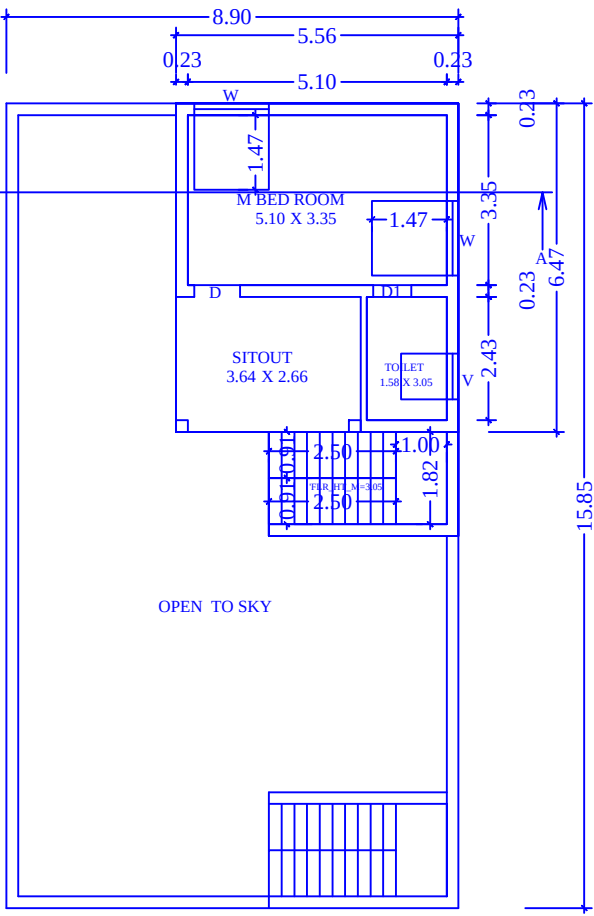
PLAN FOR FIRST FLOOR
