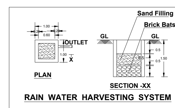
PLAN RAIN WATER HARVESTING SYSTEM
