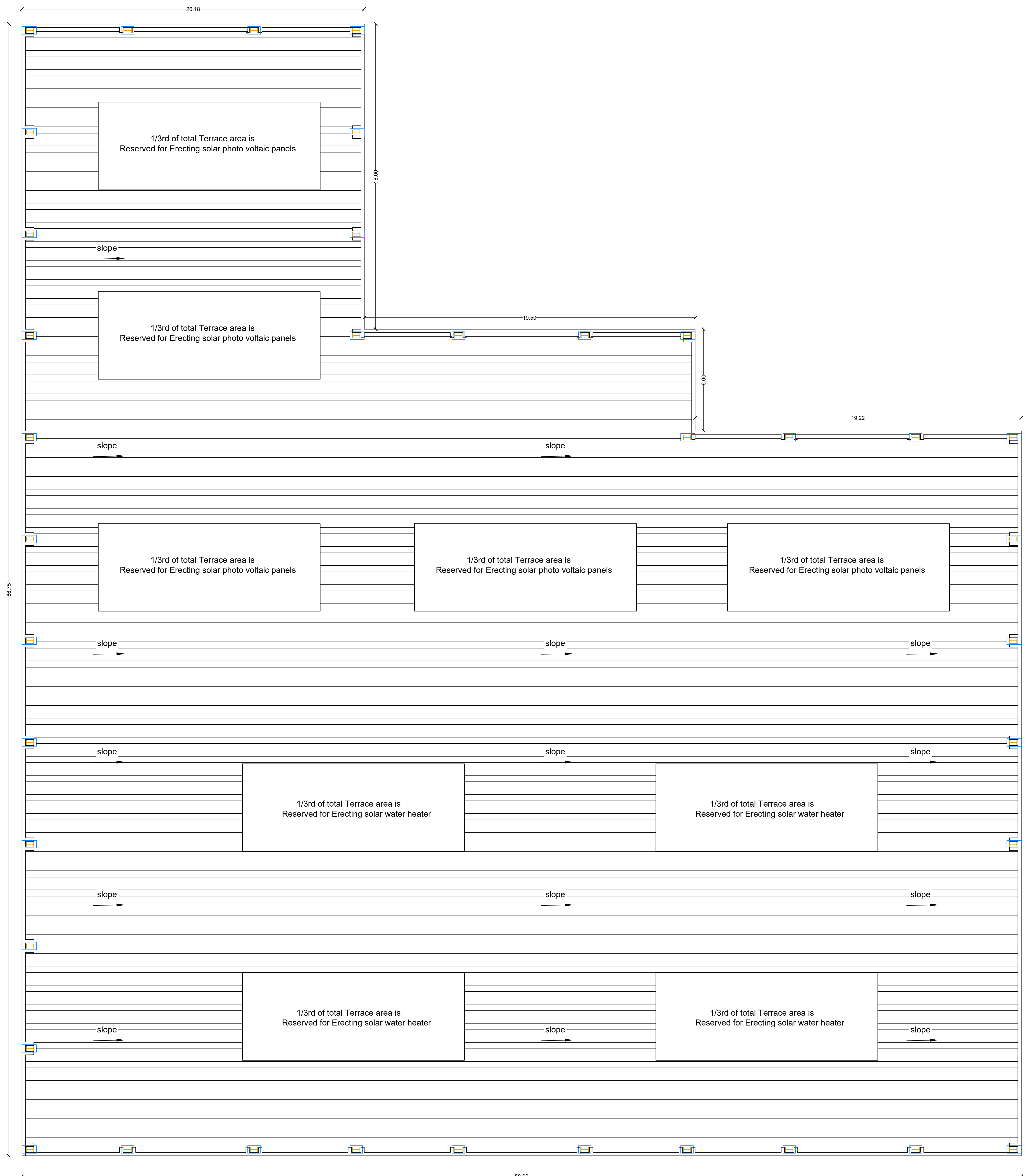
OPEN TERRACE PLAN BLOCK -1
