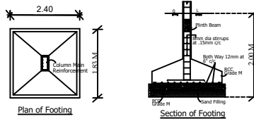
FOUNDATION DETAILS
