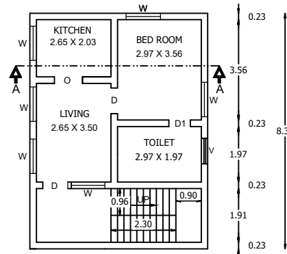
TYPICAL BLOCK 1,2 FIRST FLOOR
