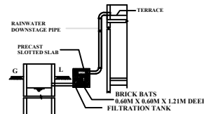
RAIN WATER HARVESTING SYSTEM
