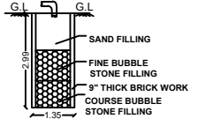
SECTION ON RAIN WATER COLLECTION TANK
