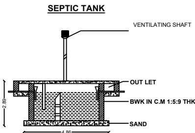
SECTION OF THE SEPTIC TANK
