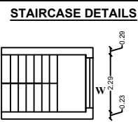
STAIRCASE DETAILS
