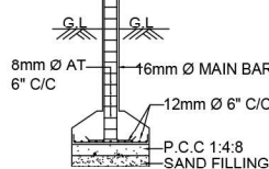
Column Footing Details: Column size - 9" x 12"
