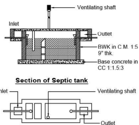
SEPTIC TANK DETAIL
