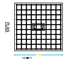
COLOUMN FOUNDATION C
